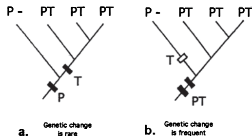
FIGURE 3. Alternative models to explain a phylogeny in which females of the least derived species have a preference "P" for a male trait "T" which occurs only in the more derived species. a) Assuming that genetic change is rare (i.e. parsimony), the preference evolved before the trait. b) Assuming that genetic change is frequent, the preference and the trait may have coevolved but the trait has subsequently been lost, probably due to selection (see explanations in the text).
