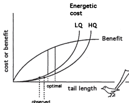
FIGURE 2. Expected optimal tail length of low quality (LQ) and high quality (HQ) males, based on the assumption that the cost of the tail is energetic, in relation to the observed tail length of these males in nature. The hypothetical case illustrated here suggests that energetic cost alone cannot account for the honesty of long tails as a signal. To simplify the illustration, the energetic cost, and the benefit of a tail are translated into the same units of fitness (e.g. number of offspring), allowing to present the case as in an additive model (see comment in legend to Fig. 1).
