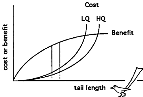
FIGURE 1. Optimal tail length for a low quality male (LQ) and for a high quality male (HQ) when a long tail is a handicap (see explanations in the text). Cost and benefit are measured using the same units of fitness (e.g. number of offspring). This allows to illustrate the handicap mechanism as in an additive model. It should be noted, however, that the actual functions creating the cost and the benefit curves might be multiplicative rather than additive (see, for example, Nur & Hasson, 1984).
