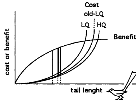
FIGURE 4. "Cheating" by an old male: If the cost of a given tail length decreases in old age, the optimal tail length for an old low quality male (Old LQ) may be higher than that of a low quality young male (LQ) and similar to that of a high quality young male (HQ). See text for more explanations. To simplify the illustration, cost and benefit are measured using the same units of fitness (e.g. number of offspring), allowing to present the case as in an additive model (see comment in the legend to fig. 1).
